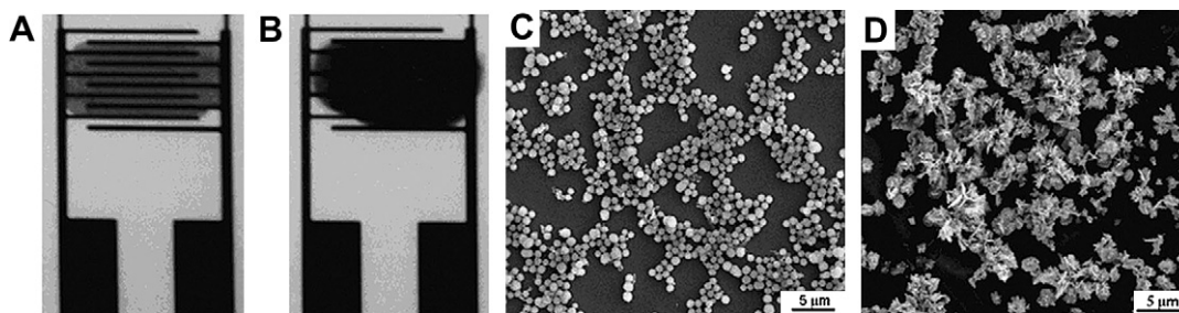
Fig. 4. Microscope (A, B) and SEM images (C, D) of the sandwich structure formation. Microscope images of ricin-containing samples (B) were heavily darkened relative to controls (A). SEM observations of particulate bridges demonstrated that MNPs from experimental groups (D) formed sandwich clusters whilst control MNPs did not (C).
