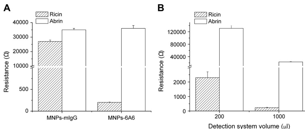
Fig. 5. (A) The specificity of SEIA using IDAMs as electrodes for ricin electrical detection. A marked electrical signal was observed in the presence of 0.1 \text{ nM} ricin, but no electrical response was observed for abrin. MNPs labeled with non-specific mIgG failed to cause any electrical signal. (B) Effect of the enrichment property of MNPs on the sensitivity of SEIA. The MNPs could successfully enrich the target and enhance the electrical signal. Error bars shown represent the standard error derived from three repeated measurements.
