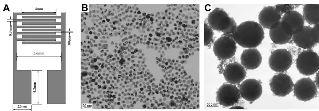
Fig. 3. (A) Diagram of the IDAMs with five pairs of 300 \mu m wide, 4000 \mu m long gold electrodes separated by a gap of 100 \mu m. TEM images of GNPs (B) and MNPs (C). The diameters of the GNPs and MNPs were approximately 10 nm and 1 \mu m, respectively.
