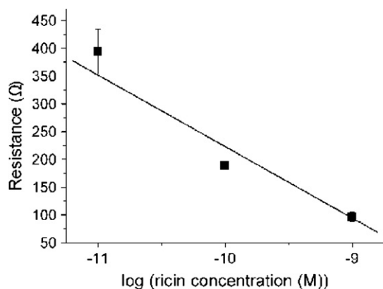
Fig. 6. The sensitivity of SEIA using IDAMs as electrodes for ricin electrical detection. A marked electrical signal was observed when ricin concentration was above 10 pM. Error bars shown represent the standard error derived from three repeated measurements.
