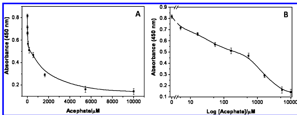
Figure 4. (A) Dose–response curve for acephate detection using the MNP peroxidase mimetic-based colorimetric assay. (B) Semilogarithmic plot of the data in panel A. The error bars represent the standard deviation of three measurements.
