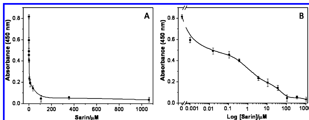
Figure 5. (A) Dose–response curve for Sarin detection using the MNP peroxidase mimetic-based colorimetric assay. (B) Semilogarithmic plot of the data in panel A. The error bars represent the standard deviation of three measurements.
