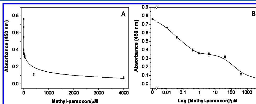
Figure 3. (A) Dose–response curve for methyl-paraoxon detection using the MNP peroxidase mimetic-based colorimetric assay. (B) Semilogarithmic plot of the data in panel A. The error bars represent the standard deviation of three measurements.
