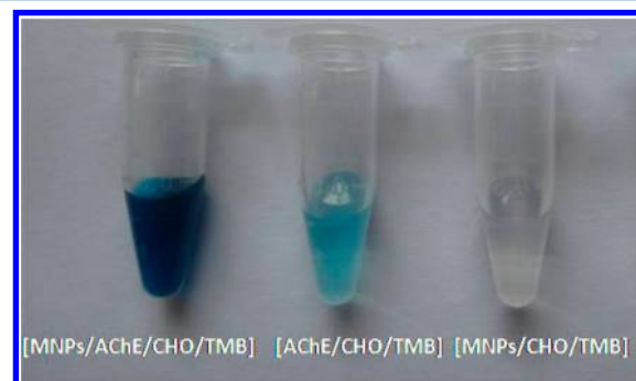
Figure 1. MNPs catalyzed the oxidation of colorimetric substrate TMB to produce a color reaction in the presence of AChE and CHO after incubation in acetylcholine chloride solution.
